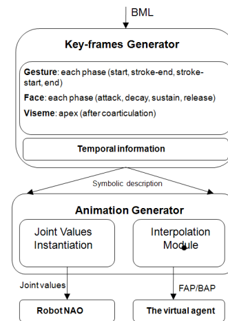
Figure 11: Two layers of Behavior Realizer.
